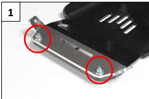
PM03-04-113 + 2 Tfhc 6x20mm + 2 M6 Washers + 2 Em6f
