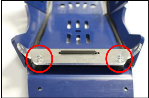
2 Tfhc 6x35mm + 2 Em6f + 2 M6 Washers
