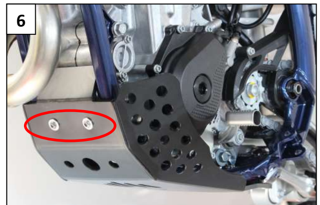
6 2 Alloy spacers + 2 Tbhc 6x35mm
