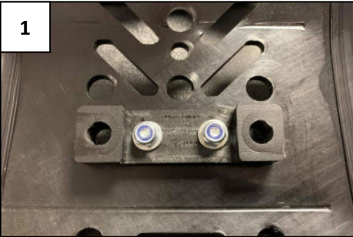
1 PM01-05-012 + 2 TFHC 6x20 + 2 R.M6 + 2 Em6f
