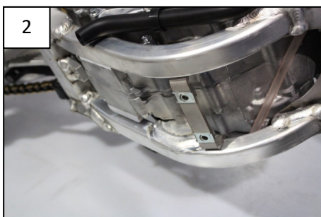
Put the front bracket in place Mettre la bride en place
