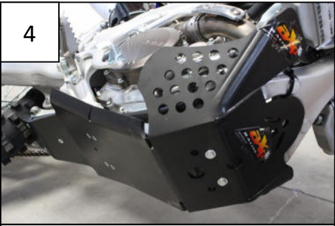
Install the plate and fit the front Th 6x25mm + NE10-01-004
