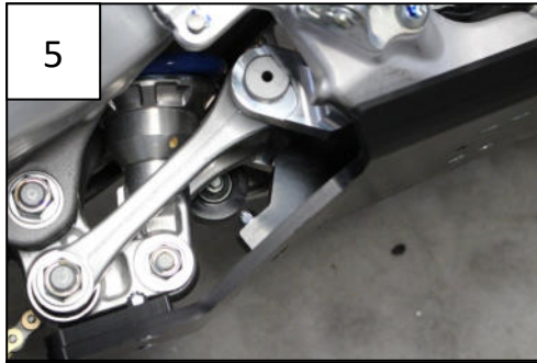
Secure the rear with PM01-04-166 + Tfhc 6x30mm + Alu ring + Em6f
