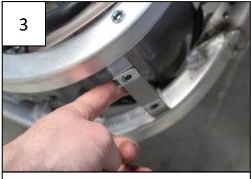
Intsall the front bracket PM02-07-008 + Clamped bolt
