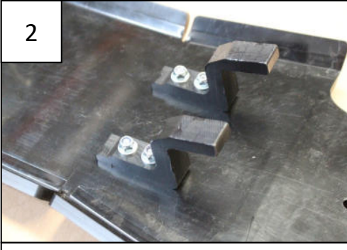
Fit PM01-04-165 Tfhc 6x25mm + Tfhc 6x40mm + Em6f + Alu rings
